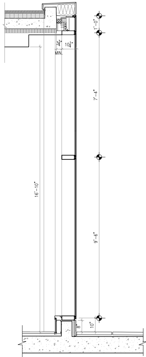
GLAZING WALL SECTION SCALE: 1/4" = 1'
